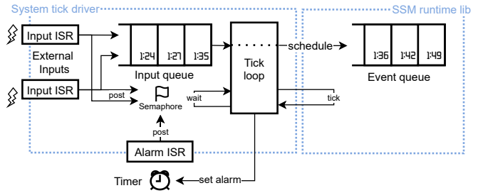
Fig. 9: The SSM runtime’s input handling architecture.
